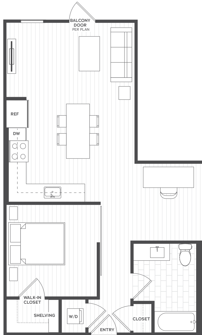
FLOORS 4-6
